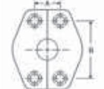
4-Bolt Split Flange
