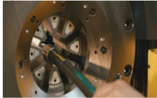
Crimp the hose/fitting assembly.
